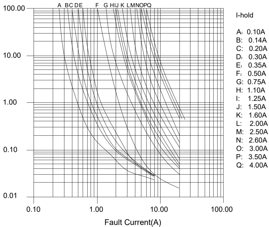
1812 Series TTT Vs Fault current chart
